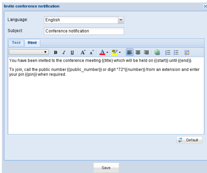
Figure 5.34: Customizing notification.
