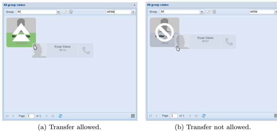
Figure 12.16: Transfer call to user via drag&drop.
