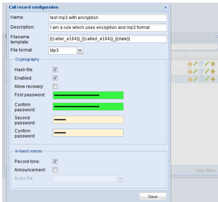
Figure 18.2: Call recording configuration edit window.
